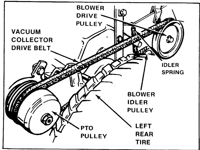
Figure 2. Drive Belt
